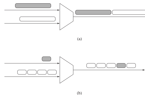
Fig. 15.2: Latency: (a) Serialization delay in a normal packet switching network. (b) Lower latency in a cell network.
