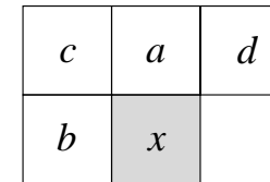
Fig. 9.14: JPEG-LS Context Model.
