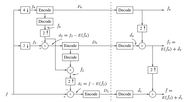
Fig. 9.5: Block diagram for Hierarchical JPEG.
