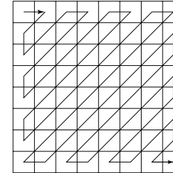
Fig. 9.4: Zig-Zag Scan in JPEG.
