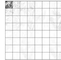
Fig. 9.7: Code block structure of EBCOT.
