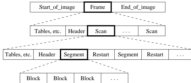
Fig. 9.6: JPEG bitstream.
