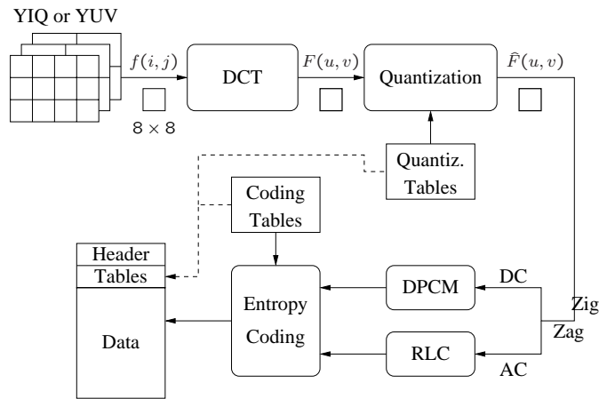
Fig. 9.1: Block diagram for JPEG encoder.
