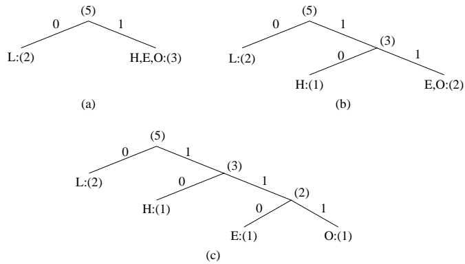
Fig. 7.3: Coding Tree for HELLO by Shannon-Fano.
