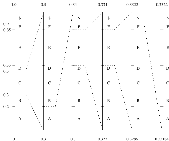
Fig. 7.8(b) Graphical display of shrinking ranges.
