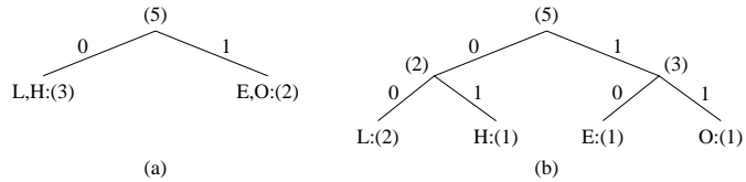
Fig. 7.4 Another coding tree for HELLO by Shannon-Fano.
