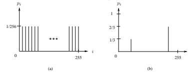
Fig. 7.2 Histograms for Two Gray-level Images.
