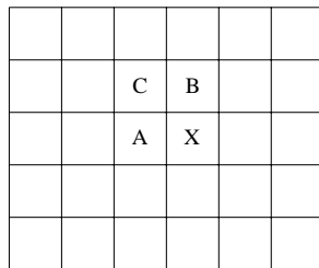
Fig. 7.10: Neighboring Pixels for Predictors in Lossless JPEG.
