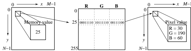
Fig. 3.8: Color LUT for 8-bit color images.
