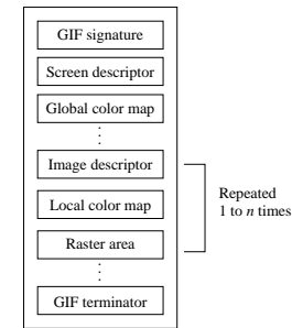
Fig. 3.12: GIF file format.
