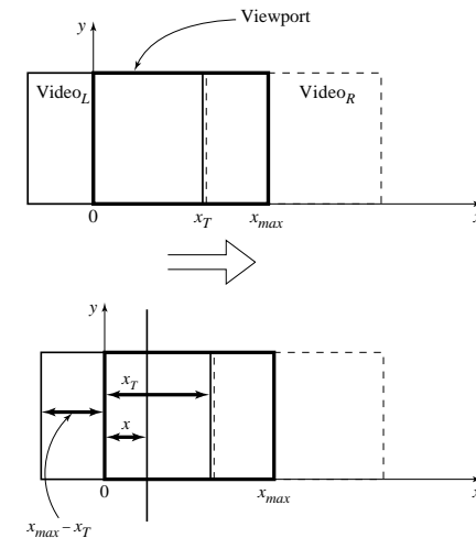
Fig. 2.10: (a): Geometry of Video L pushing out Video R . (b): Calculating position in Video L , from where pixels are copied to the viewport.
