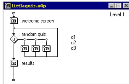
Fig. 2.1: Authorware flowchart
